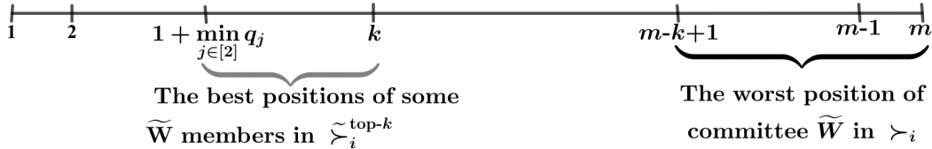
Figure 2: Positions of \widetilde{W} members before and after the top- k -position constraint
